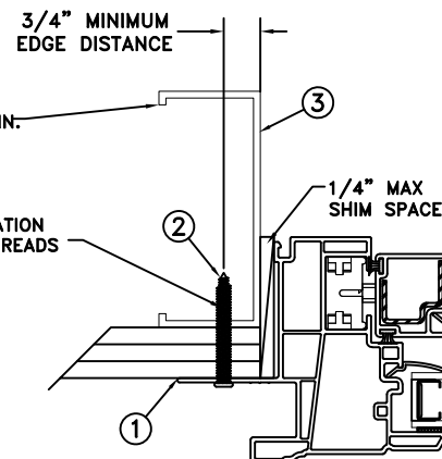
FRAME JAMB SECTION (TYP) HORIZONTAL SECTION
